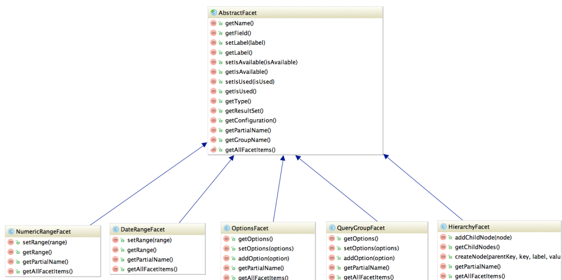
Figure 11.2: UML diagram of the *Facet classes
