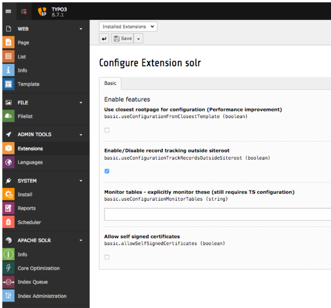
Figure 5.3: Enable tracking of records outside siteroot
